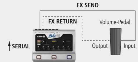
Fig. 3: Volume pedal as Master Volume
